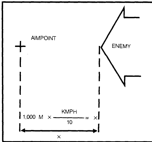
Figure 6-6. AIMPOINT LOCATION FOR MOVING TARGETS
