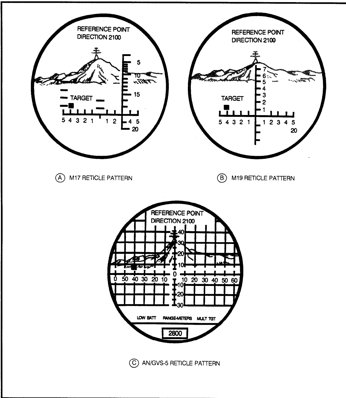
Figure 3-6. MEASURING ANGULAR DEVIATIONS WITH BINOCULARS AND AN/GVS-5
